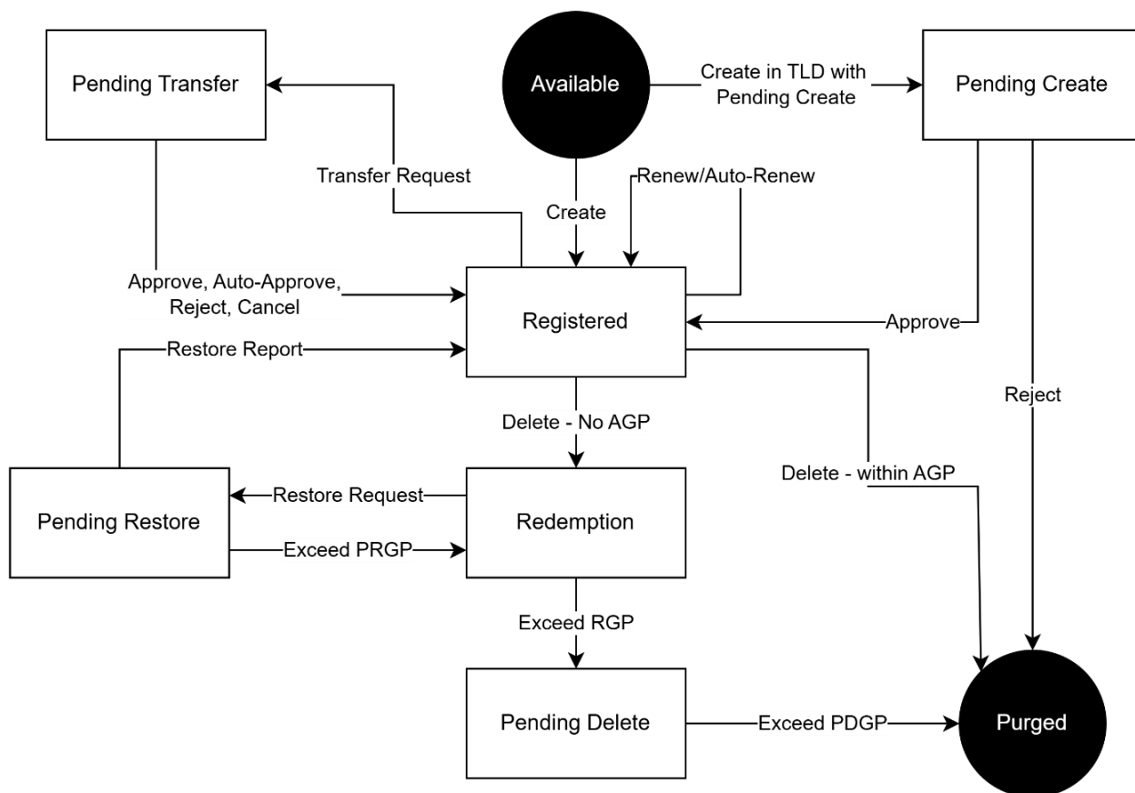
Figure 1: Domain Status with Grace Period
